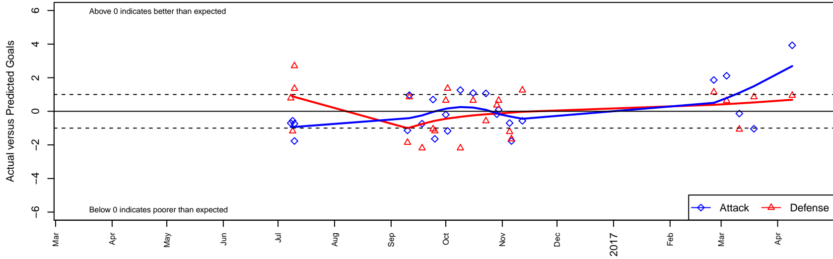
PCU Red 2 G05 Dots are actual minus expected GF (blue circles) and GA (red triangles). Blue line is smoothed change in attack strength. Red is smoothed change in defense strength.
